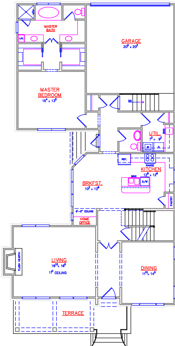
VILLAGE A - 90' FIRST FLOOR PLAN
