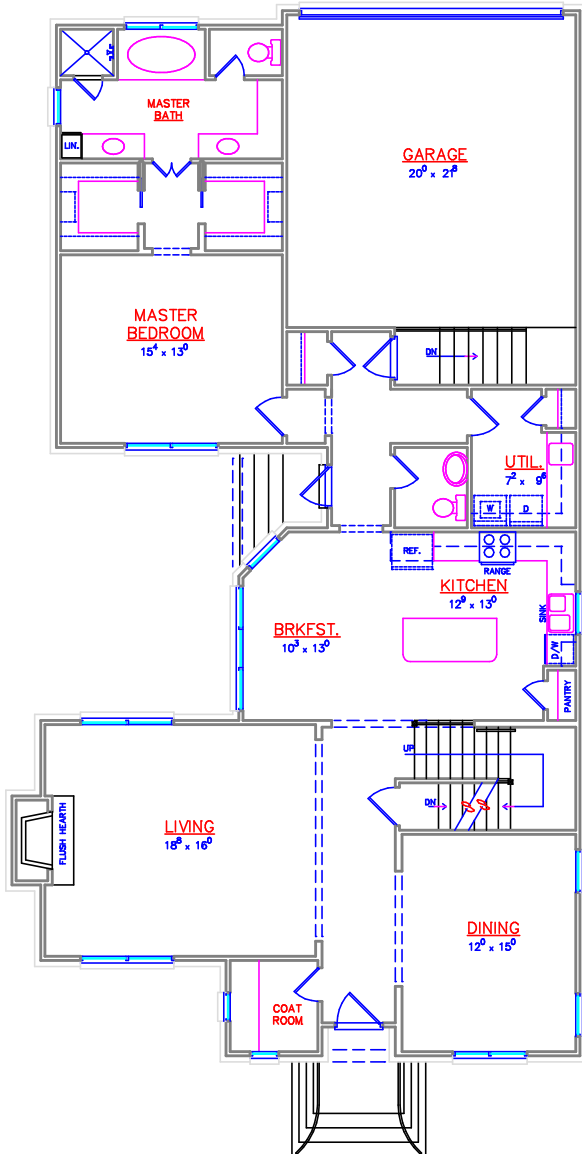
VILLAGE A – ALTERNATE FIRST FLOOR PLAN
