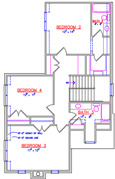
VILLAGE B – INTEGRAL SECOND FLOOR PLAN
