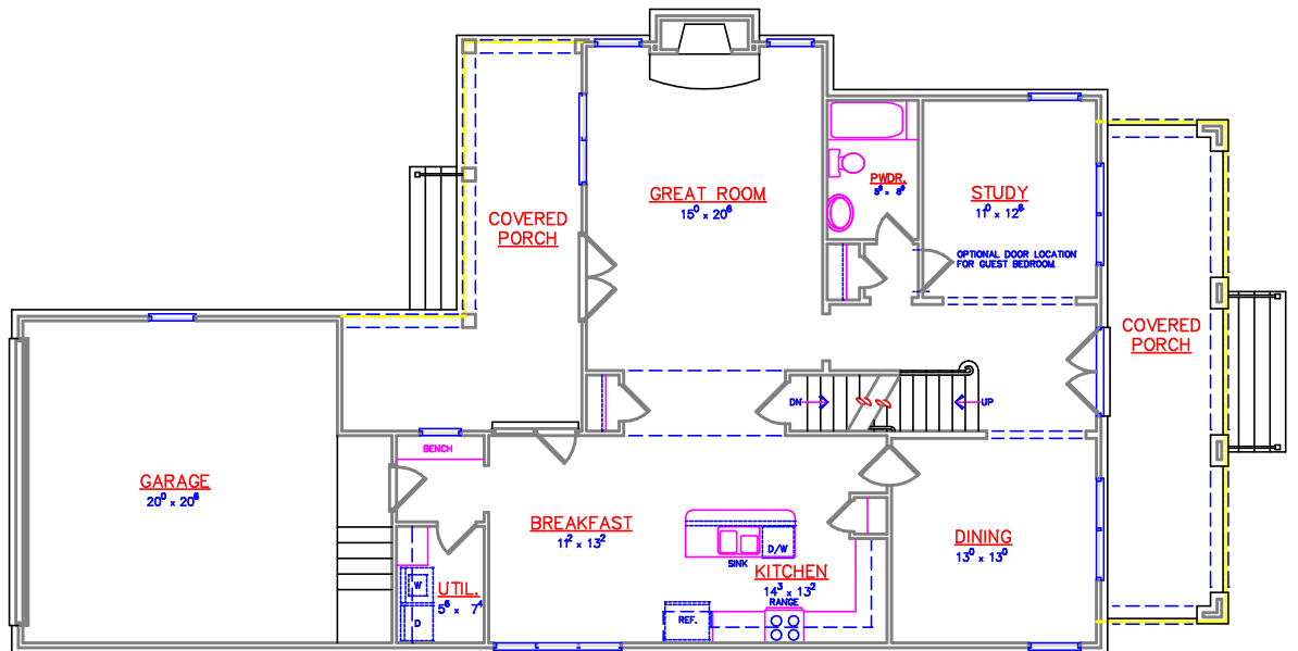
VILLAGE C - 90' FIRST FLOOR PLAN
