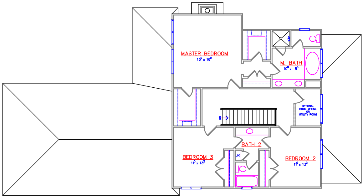
VILLAGE C - 90' SECOND FLOOR PLAN
