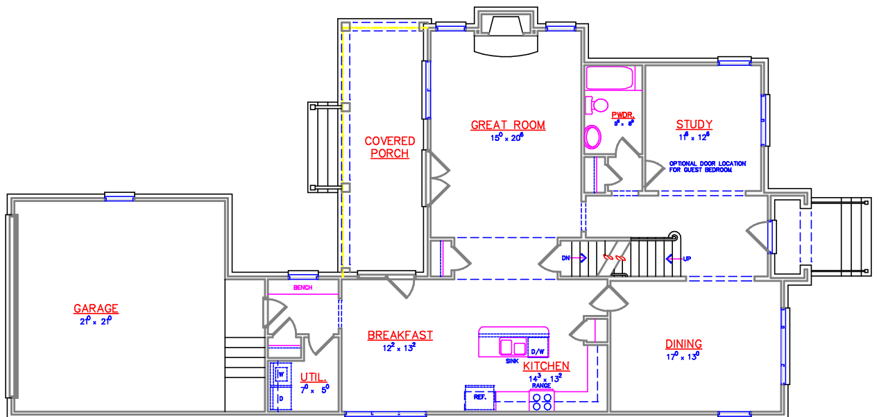
VILLAGE C – ALTERNATE FIRST FLOOR PLAN
