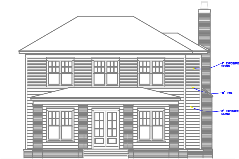
VILLAGE C – INTEGRAL FRONT ELEVATION
