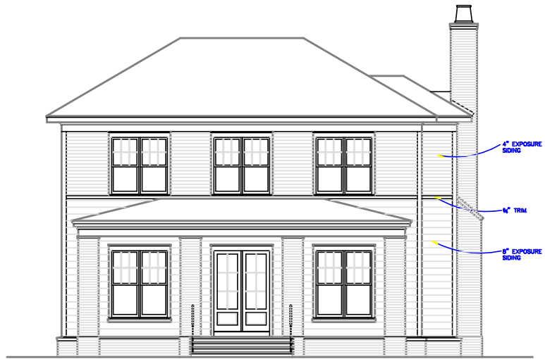
VILLAGE C – CRAWLSPACE/NO GARAGE FRONT ELEVATION
