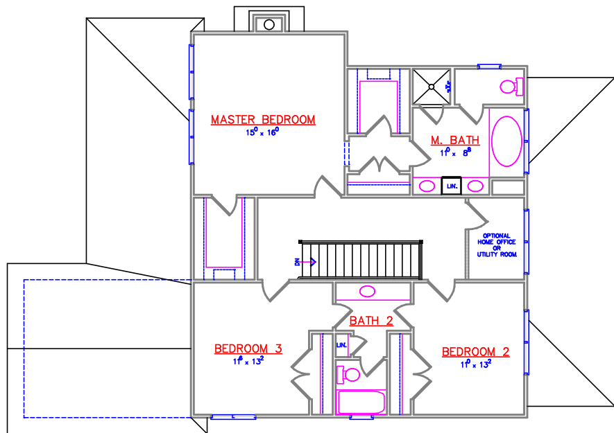
VILLAGE C – CRAWLSPACE/NO GARAGE SECOND FLOOR PLAN
