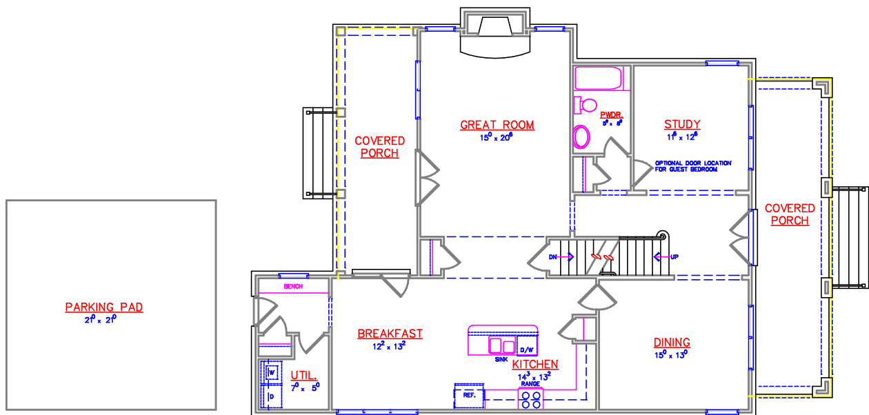
VILLAGE C – CRAWLSPACE/NO GARAGE FIRST FLOOR PLAN
