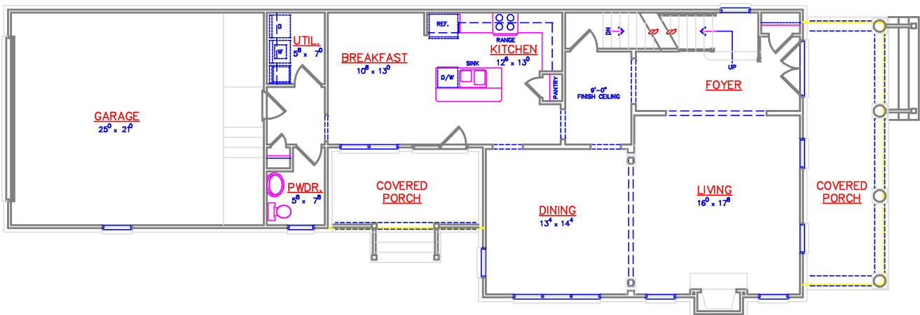
VILLAGE D – ALTERNATE FIRST FLOOR PLAN
